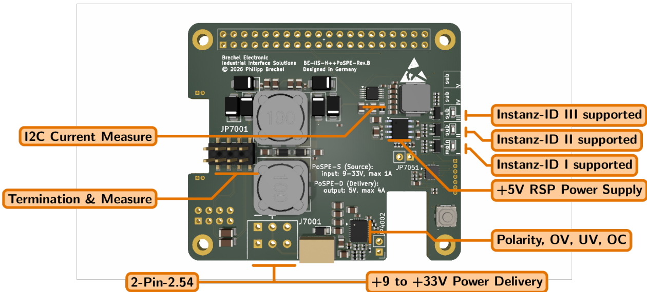
Figure 1: BE-IIS-PoSPE top view with annotations
