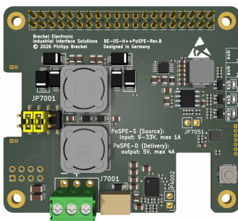
Figure 3: JP7001 jumper configuration with SPE termination enabled. The highlighted jumpers indicate bus end node configuration.
