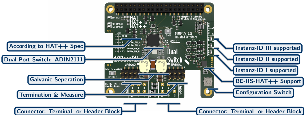
Figure 2: BE-IIS-HPP-2T1L Industrial HAT with annotations
