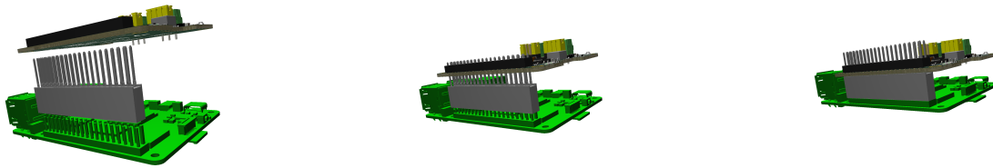
Figure 9: Assembly of the 2x20-pin stackable header between Raspberry Pi and HAT
